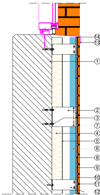
Window Bottom Connection Section
