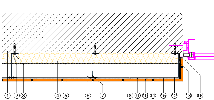
Window Edge Connection Plan
