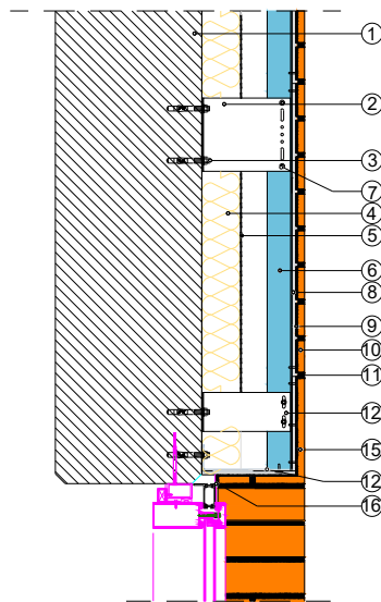
Window Top Connection Section
